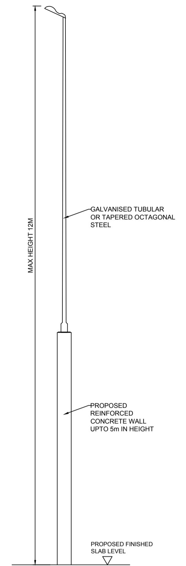
LAMP POST TYPICAL DETAIL SCALE 1:50
